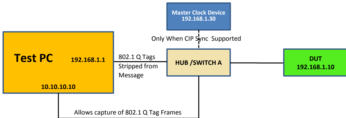
Figure 2: Test setup for QoS Object PTP DSCP and 802.1 Q Tagging Test
