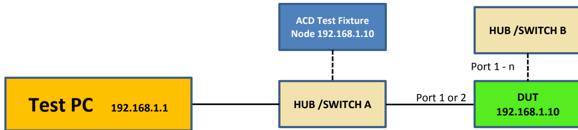
Figure 1: Test setup for all Test Cases
